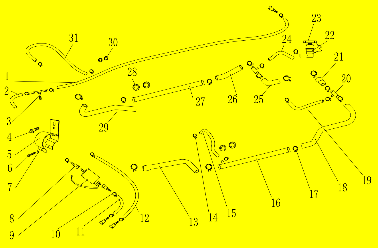
WATER PIPE & THREE-WAY
