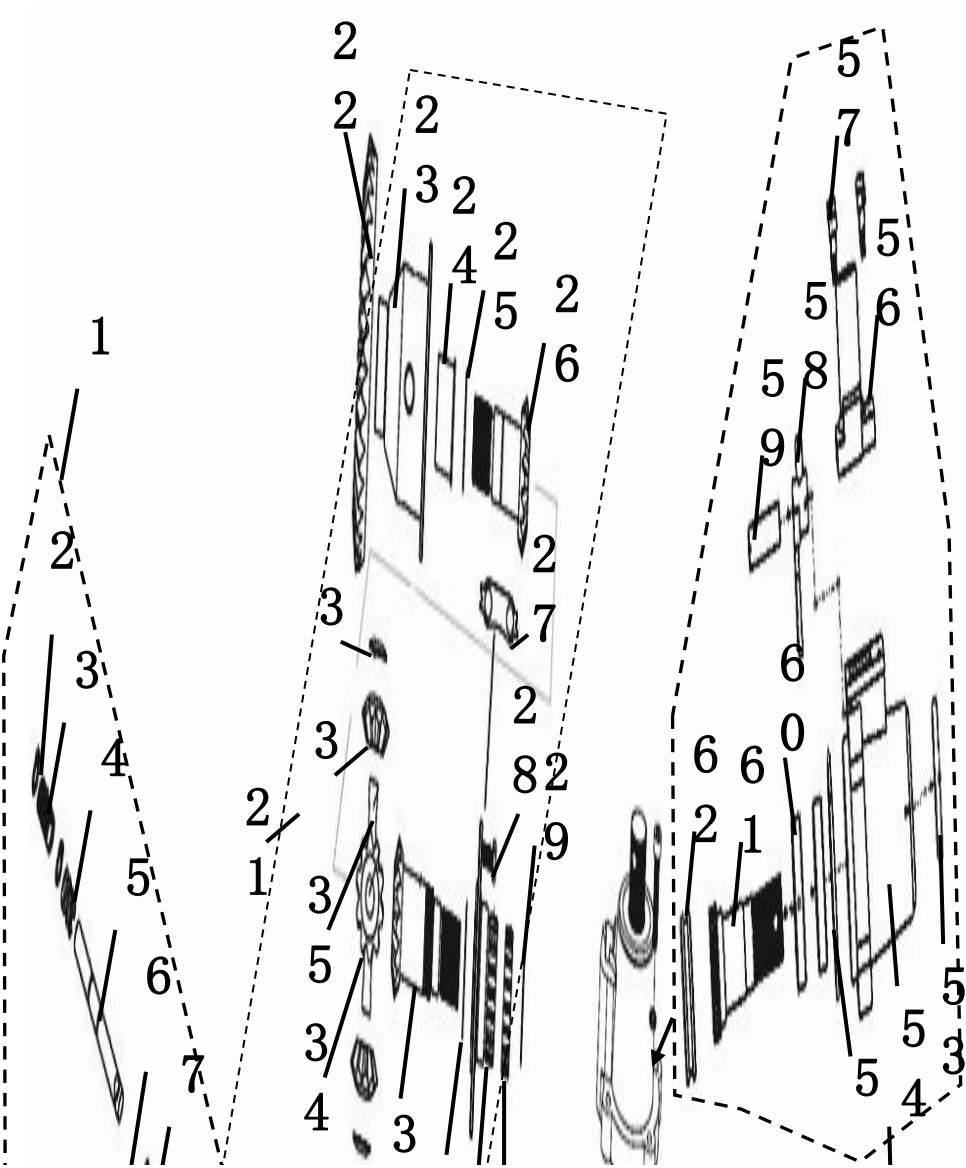
F-16 前桥总成—FRONT AXLE ASSEMBLY
