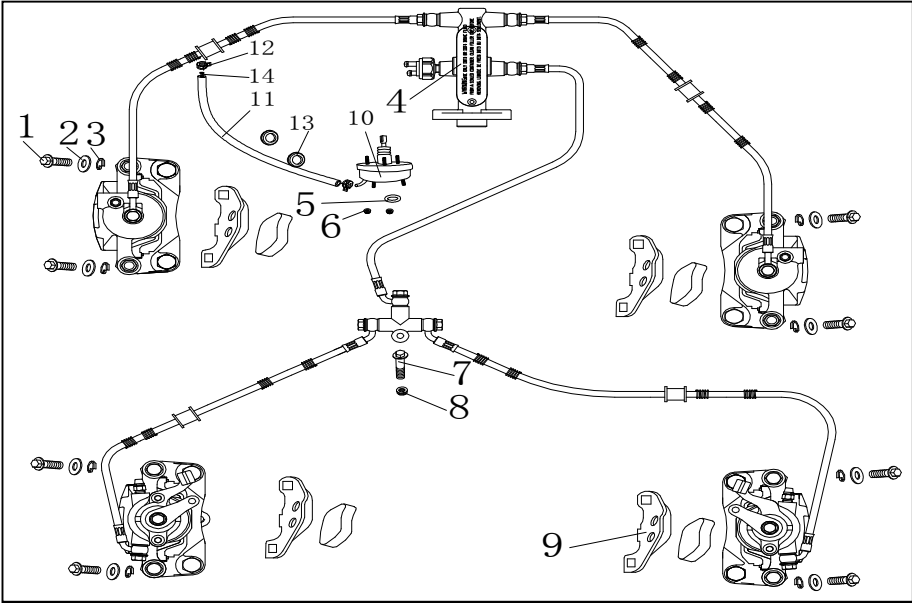
F-9 制动系统---BRAKING SYSTEM
