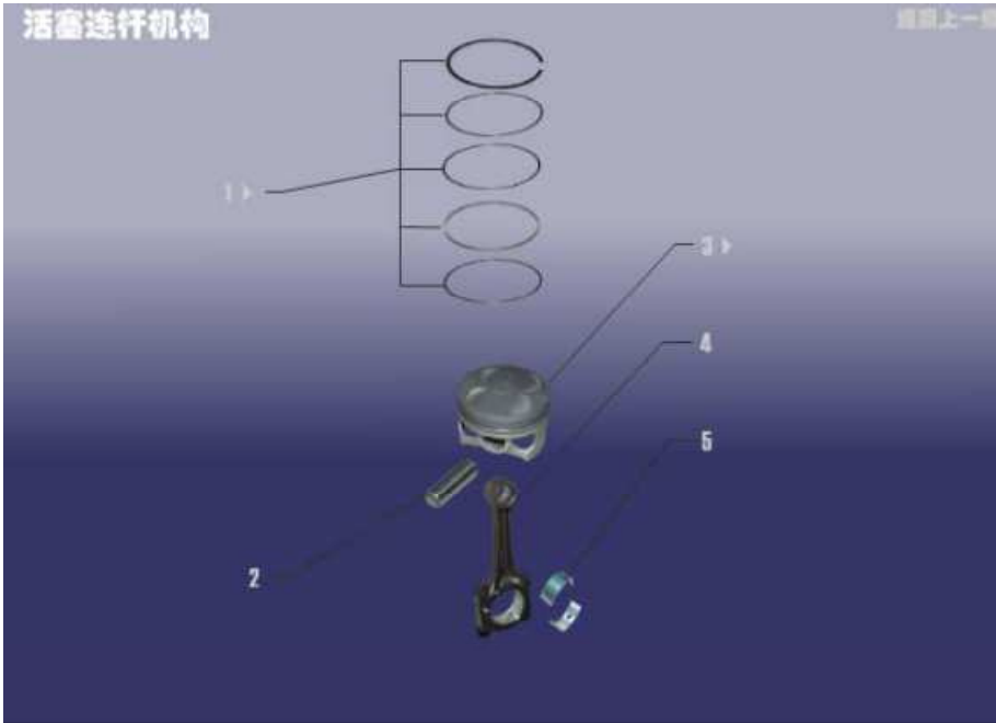
E-3 活塞连杆机构---PISTON CRANK MECHANISM
